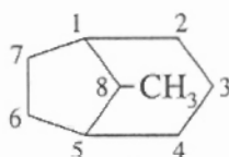
8-Methylbicyclo[3.2.1]octane
