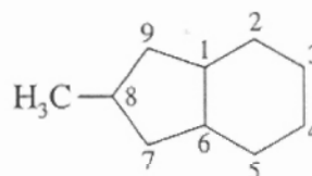
8-Methylbicyclo[4.3.0]nonane
